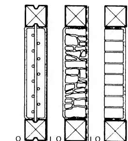
11 Panel built up with earth and wooden canes, filled in with building rubble, with klinker nogging
